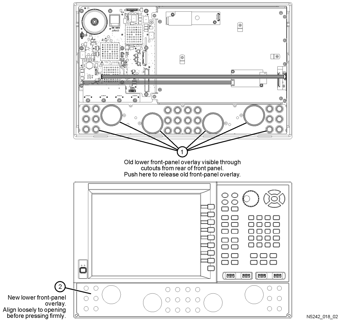
Figure 15 Lower Front Panel Overlay Replacement
